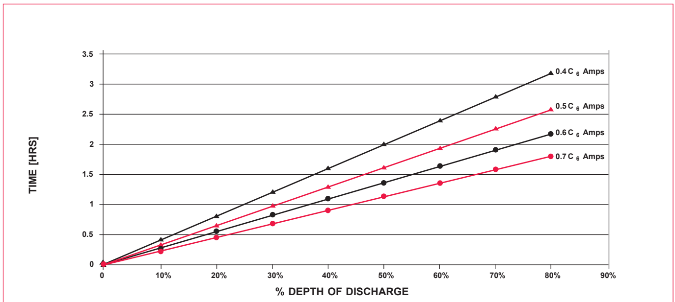
Figure 4 – Recharge time – return 100% of discharged Ah's
