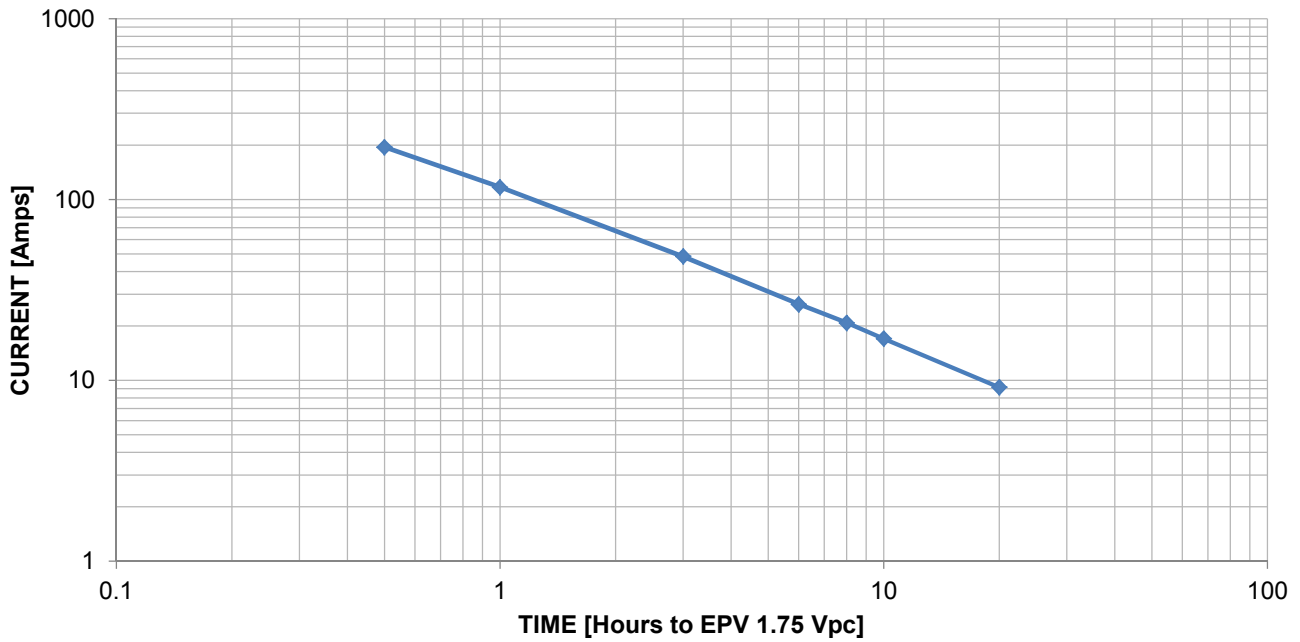
12NXS158 Performance data @ 77°F (25°C)
