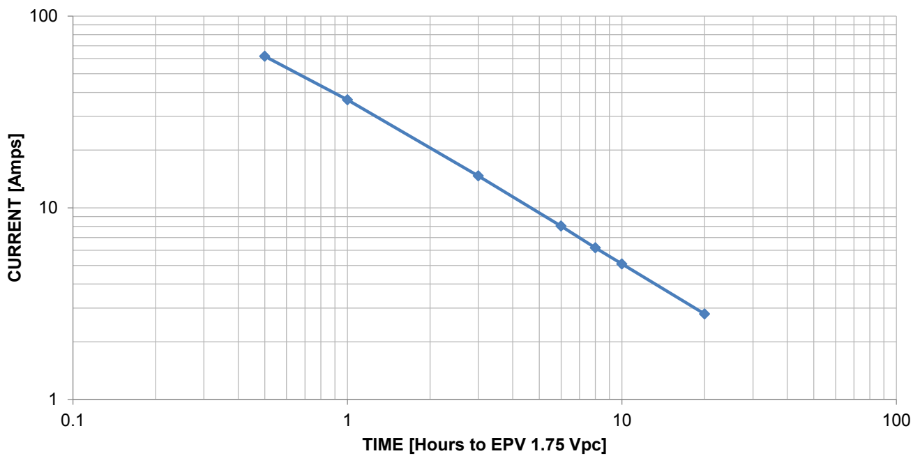
12NXS50 Performance data @ 77°F (25°C)
