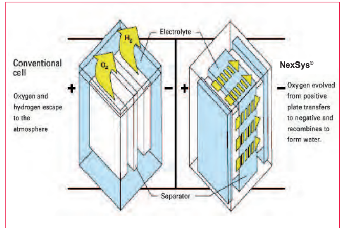
Figure 1 - Principle of the oxygen reduction cycle
