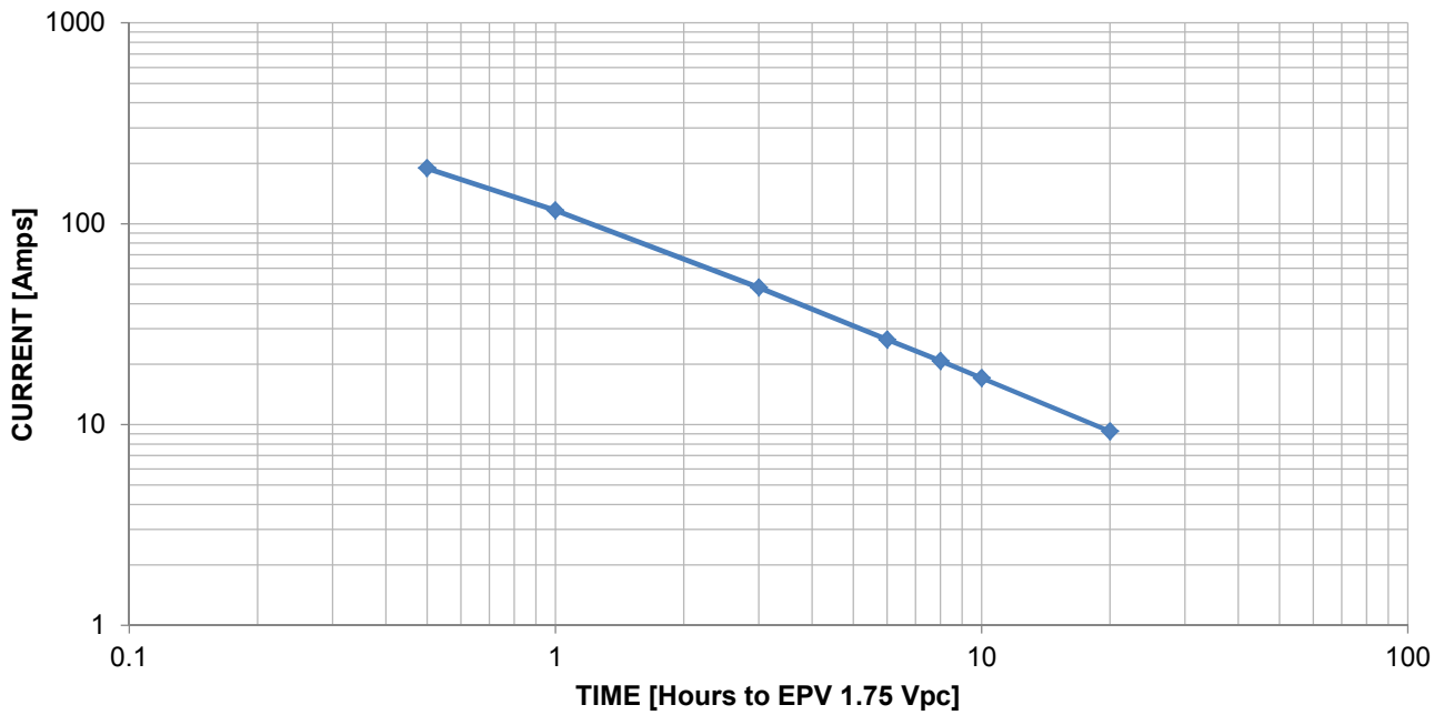
12NXS166 Performance data @ 77°F (25°C)
