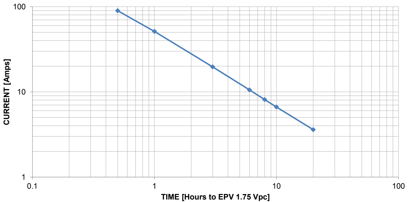
12NXS62 Performance data @ 77°F (25°C)
