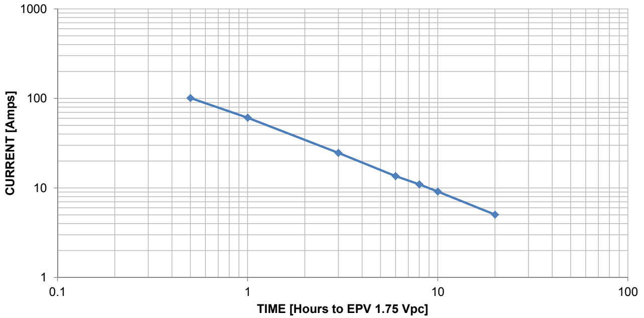
12NXS85 Performance data @ 77°F (25°C)
