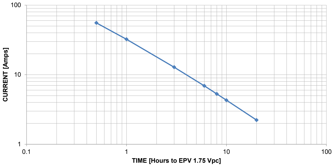
12NXS38 Performance data @ 77°F (25°C)
