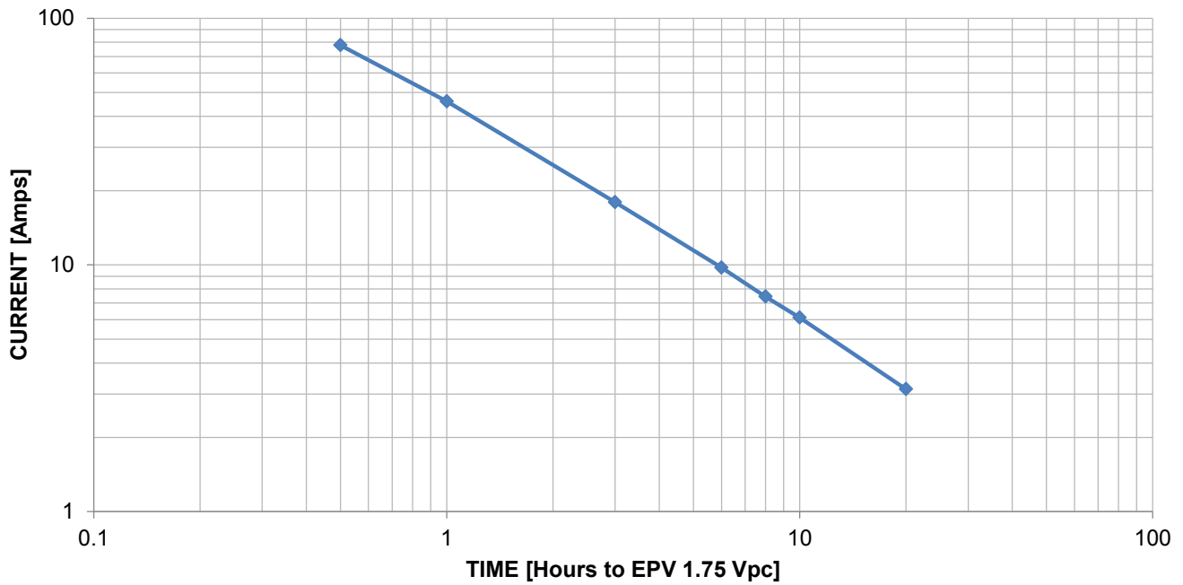
12NXS61 Performance data @ 77°F (25°C)
