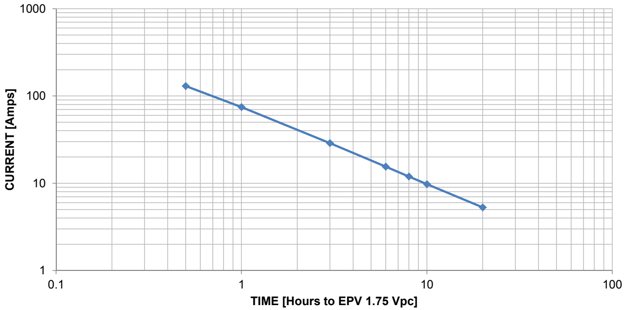
12NXS89 Performance data @ 77°F (25°C)
