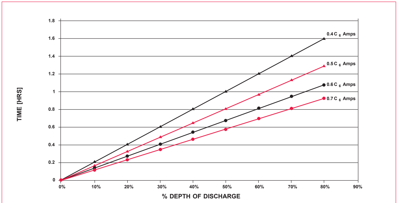
Figure 3 – Recharge time – return 80% of discharged Ah's
