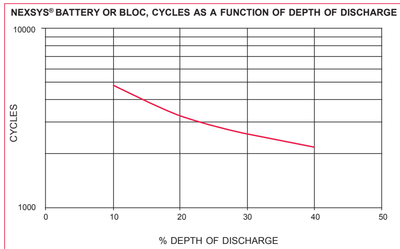
Figure 5 - Cycle Life as a Function of Depth of Discharge 10%-40% ( C_6 Rate)
