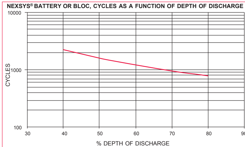
Figure 6 - Cycle Life as a Function of Depth of Discharge 40%-80% ( C_6 Rate)
